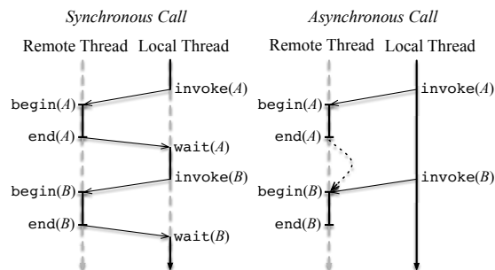
Figure 1: Synchronous versus asynchronous events.
