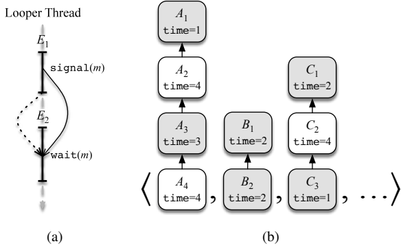
Figure 8: (a) Illustration of Rule ATOMIC. (b) Illustration of async-before lists for Delayed events. The causal predecessors of an event with time = 3 are shown in gray.
