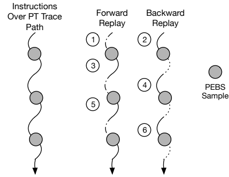
Figure 4: Forward and Backward Replays.
