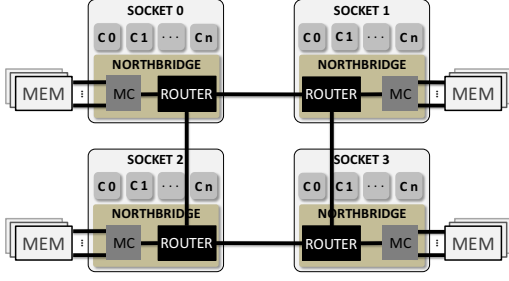
Figure 1. Block diagram of a 4-socket server system
