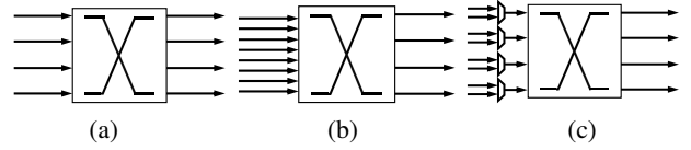
Figure 2. Block diagram of (a) conventional 4-port router, (b) integrated 2-way concentration, and (c) external 2-way concentration router.
