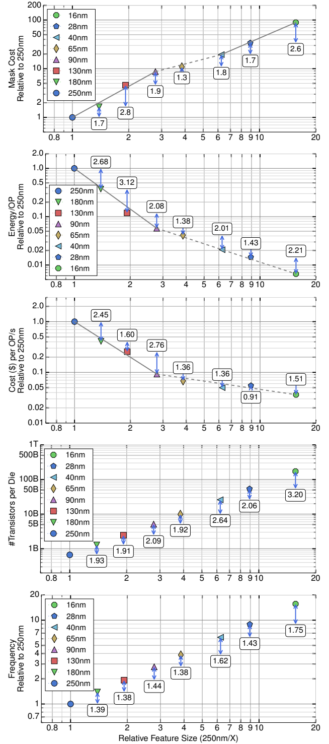
Figure 1: Node Technology trade-offs, normalized to 250nm. #'s indicate multiplicative benefits as node advance. Lines in mask cost indicate different regimes of mask cost scaling. The dotted lines in energy and cost per op/s graphs indicate the post-Dennard slowdown in voltage scaling.
