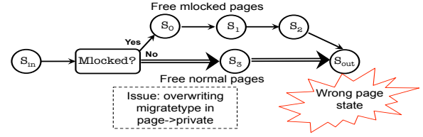
Figure 3. A bug caused by overwriting the immutable variable migratetype in the fast path for memory allocation.
