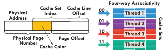
Figure 3. Page coloring.
