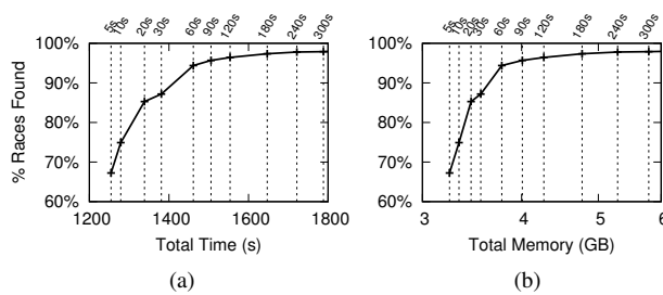
Figure 10: The percentages of races reported from 8 selected applications versus the total time and memory used for various time windows. The memory axis is in log scale.
