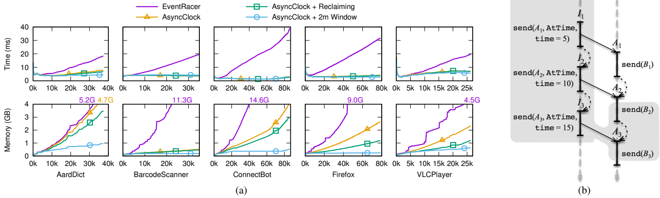
Figure 9: (a) Comparison between EVENTRACER and ASYNCCLOCK. The x-axes show the number of looper events. The top row shows the average time spent per event . The bottom row shows total memory used during the analyses. The results of 3 configurations of ASYNCCLOCK are shown: no event reclaiming ( \triangle ), reclaiming heirless events ( \square ), and reclaiming events with a 2-minute time window ( \circ ). (b) An event pattern in BarcodeScanner, where I_n are input events. EVENTRACER traversed the shaded area to find predecessors of B_3 .
