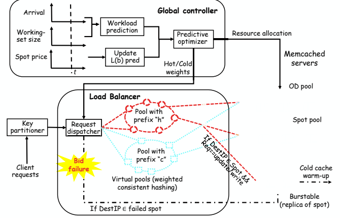
Figure 6: Key elements of our prototype implementation.
