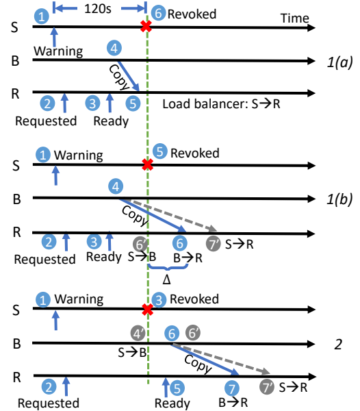
Figure 4: Different cases for the failure recovery process. “S, B, R” denote spot, backup and replacement, respectively. Events 6’ – 7’: B is only used for warming up R. Events 4-7: B is used for both warming up R and serving requests.
