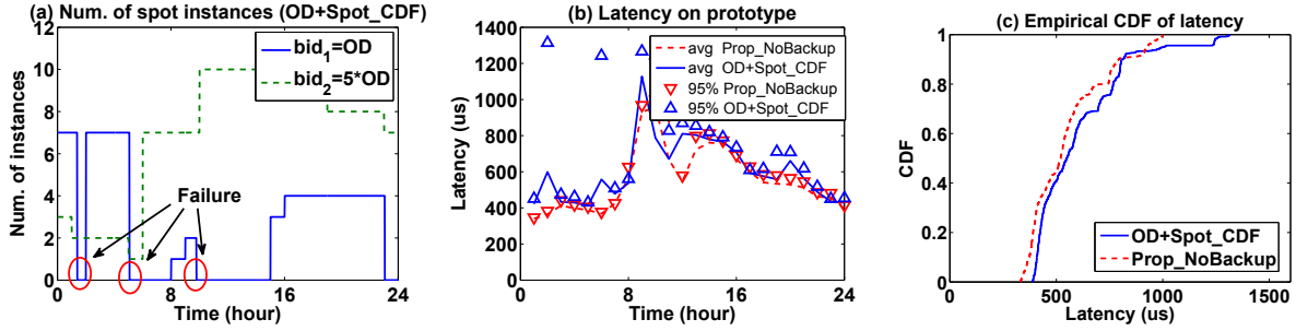
Figure 9: Resource allocation and performance measurement on EC2 (impact of spot prediction).
