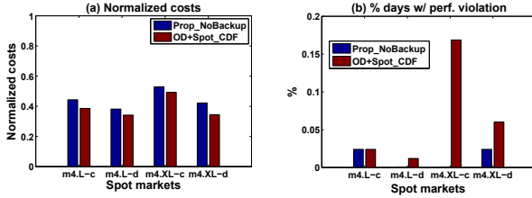
Figure 7: Normalized costs (divided by costs of ODOnly) and percentage of days when the performance target is violated when using Prop.NoBackup and OD+Spot.CDF.
