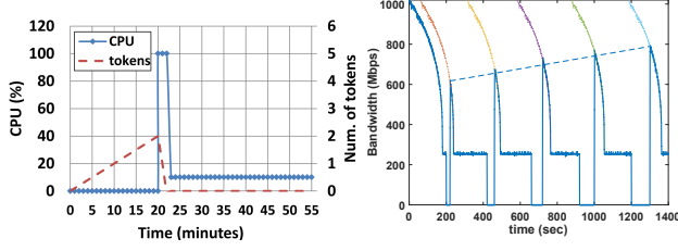
Figure 5: The token-bucket mechanisms of the CPU capacity and network bandwidth for t2.micro.
