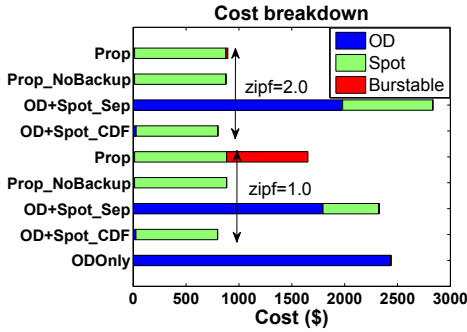
Figure 12: Long term (90-day) cost breakdown (max. arrival rate: 500kops; max. working set size: 100 GB).
