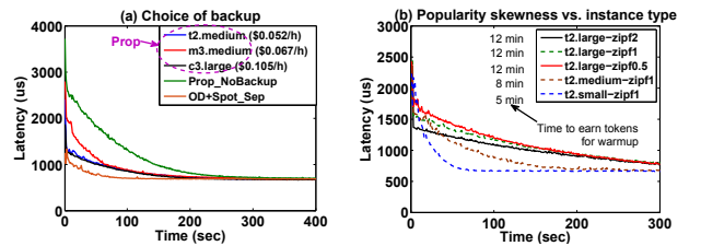
Figure 11: Recovery latency under (a) different choices of backup and (b) different content popularity distributions and instance types. The curves for t2.medium and c3.large in (a) almost fully overlap.
