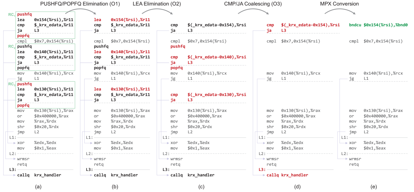
Figure 2. The different optimization phases of kR ^ X-SFI (a)–(d) and kR ^ X-MPX (e).
