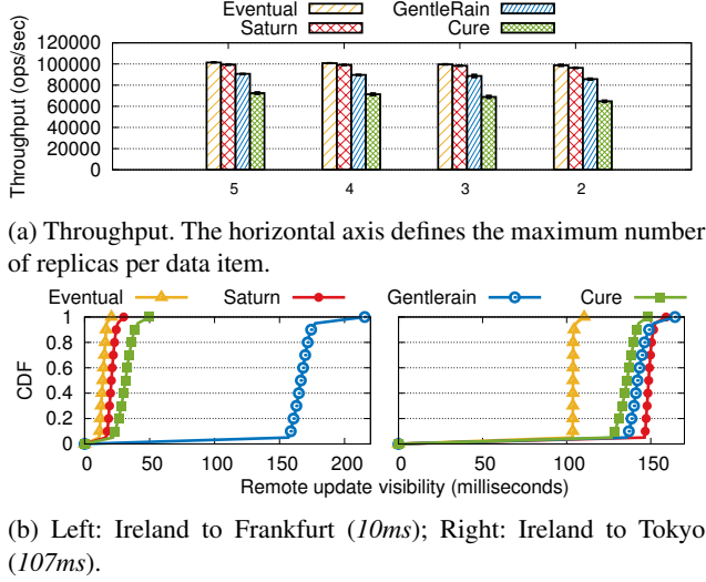
Figure 8: Facebook-based benchmark results.
