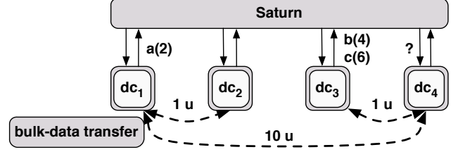
Figure 3: Label propagation scenario.
