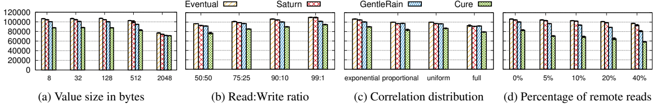
Figure 5: Dynamic workload throughput experiments.
