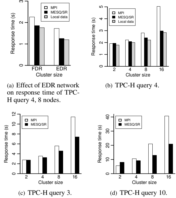
Figure 14. TPC-H query response time, 100 GiB per node.
