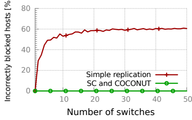
Figure 3: Simple replication causes incorrect blocking.
