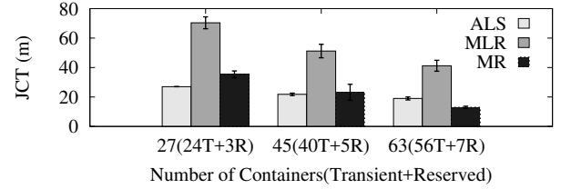
Figure 9. The job completion times of applications on Pado with different numbers of a fixed 8 : 1 ratio of transient and reserved containers under the high eviction rate
