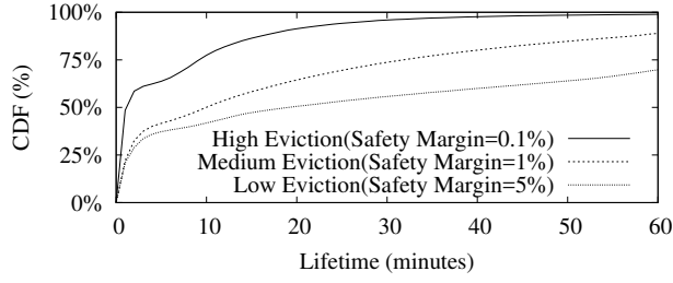
Figure 1. CDFs of transient container lifetimes over different safety margins.
