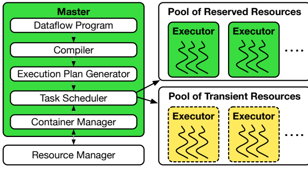
Figure 4. Pado Runtime
