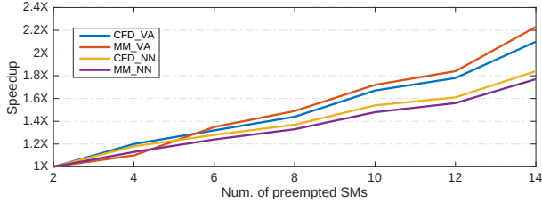
Figure 16: Performance improvement over baseline spatial preemption.
