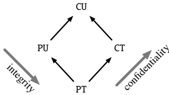
Figure 4. Security lattice for TrustZone.
