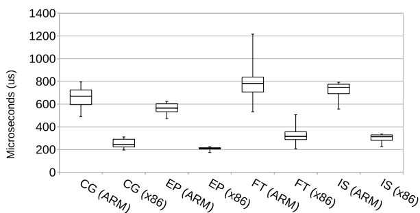
Figure 7. Stack transformation latencies. Each plot shows the minimum, 1 st quartile, median, 3 rd quartile and maximum transformation latencies experienced across all migration points for each benchmark.
