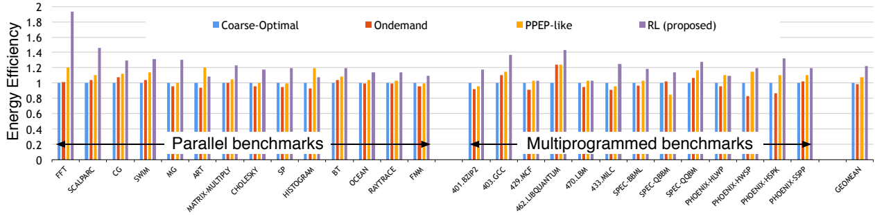
Figure 9. Energy efficiency ( 1/\text{Energy} ) normalized to the baseline “Coarse-optimal”—a coarse-grained control policy with perfect knowledge of the workloads. All policies are running on the same framework 2- N under a maximum 5% performance loss constraint.
