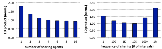
Figure 12. System ED product v.s. the number of RL sharing agents (cores), and the sharing frequency. Results are normalized to the setting (4 agents, 10K intervals) in this work.
