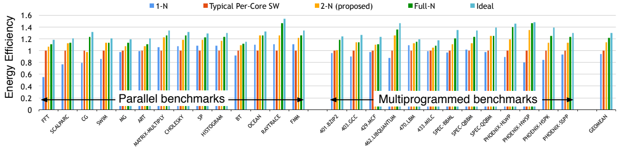
Figure 8. Energy efficiency ( 1/\text{Energy} ) under a maximum of 5% performance loss is normalized to the baseline “Typical Per-Core SW”—a framework with only on-chip switching regulators ( \eta < 80\% ). The same oracle control policy is assumed for all frameworks.
