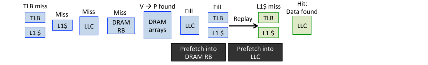
Figure 6. Timeline of events when TEMPO prefetches the data that the replayed instruction will use into the DRAM row buffer and LLC. Subsequent LLC and row buffer hits improve performance.
