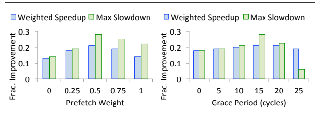
Figure 16. (Left) Fractional improvements versus the baseline, using TEMPO, in weighted speedup and maximum slowdown of any application as a function of the post-page table prefetch weight versus other memory reference; and (right) as a function of the grace period after the replay’s data is prefetched into the row buffer.
