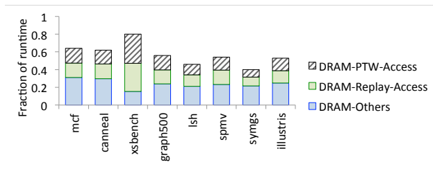
Figure 1. Fraction of total application runtime for page table accesses to DRAM (DRAM-PTW-Access), replayed accesses to DRAM (DRAM-Replay-Access), and other non-page table DRAM accesses (DRAM-Other).
