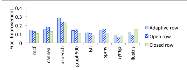
Figure 14. Performance improvements for TEMPO assuming adaptive, open, and closed-row-policies.
