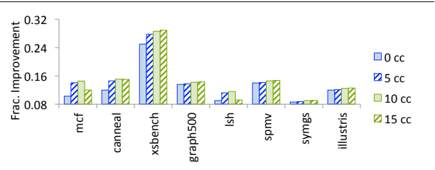
Figure 15. Performance improvements for TEMPO as the number of cycles we wait anticipating future page table accesses varies.
