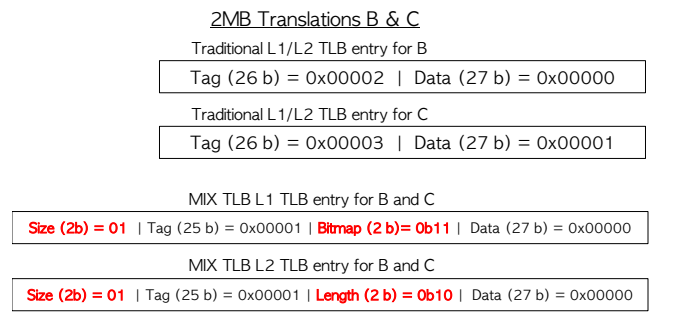
Figure 6. Traditional TLB and MIX TLB entries for the translation corresponding to 2MB pages B-C. L1 MIX TLB and L2 MIX TLB entries use a bitmap and a length field to record contiguous superpages, respectively. We assume 2-set TLBs.
