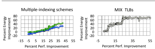
Figure 16. (Left) performance-energy tradeoffs for skew-associative TLBs with prediction (blue) and hash-rehash with prediction (green); and (Right) MIX TLB performance-energy tradeoffs.
