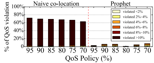
Figure 19: Percentage of QoS violation in all scheduled co-locations under each QoS policy.
