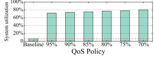
Figure 18: Accelerator utilization when using Prophet to select “safe” co-locations under each QoS policy.
