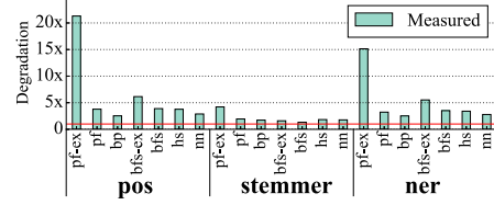
Figure 4: Performance degradation of PCIe-intensive LS applications when they are co-located with PCIe-intensive batch applications.
