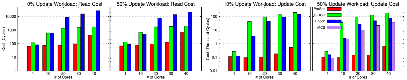
Figure 6. PARSEC \mu -benchmark: 99th Percentile Latency for Read / Update Workloads
