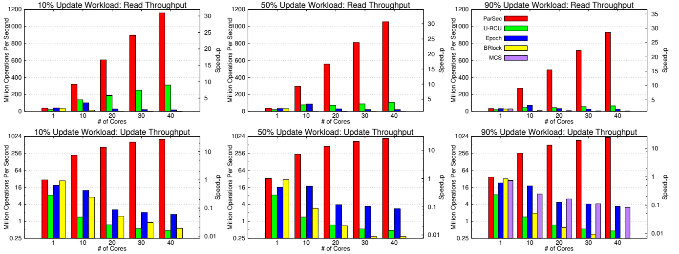
Figure 5. PARSEC \mu -benchmark: Read / Update Throughput
