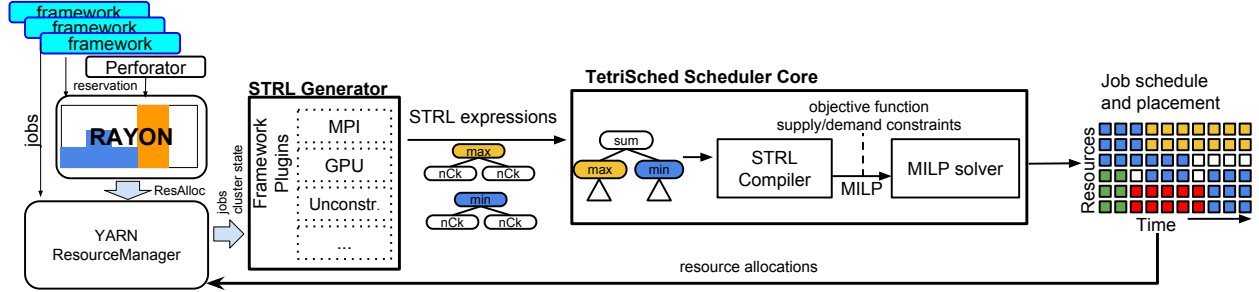
Figure 2. TetriSched system architecture
