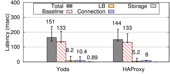
Figure 9. YODA latency breakdown.
