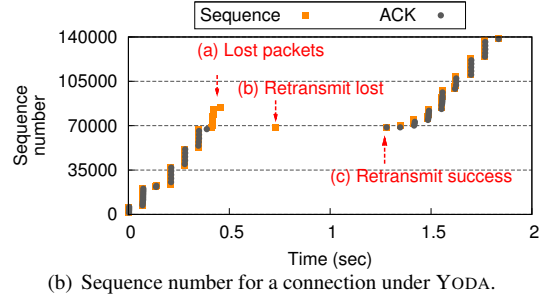
Figure 12. YODA Failure recovery.
