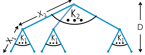
Figure 5: A simple two level hierarchy. Let X_1 and X_2 be distribution of times taken in the first and the second levels of the hierarchy, respectively.
