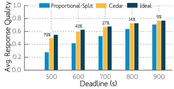
Figure 15: Improvement in Response Quality. X_1 is per Cosmos’s extract distribution and X_2 is per Cosmos’s full-aggregate distribution. The fanout at both levels is fixed at 50.
