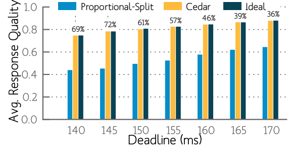
Figure 14: Improvement in Response Quality. X_1 is per Facebook’s map distribution and X_2 is per Google’s distribution. The fanout at both layers is 50.
