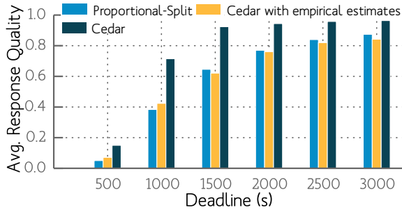
Figure 10: Spark implementation results showing that Cedar’s learning algorithm provides significant benefits over using empirical estimates for the parameters. its gains—eliminating bias in received samples using order statistics (§5.3.1); and a simple yet accurate online learning algorithm (§5.3.2).
