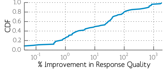
Figure 8: CDF of Percentage improvement of individual queries. The deadline is set to 1000s. We only look at queries having > 5% quality in the baseline approach to prevent improvements from being unreasonably high.
