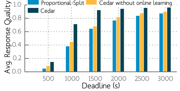
Figure 11: Spark implementation results showing that Cedar copes well with load fluctuations that can increase (or decrease) mean process durations by learning the distributions in an online fashion.
