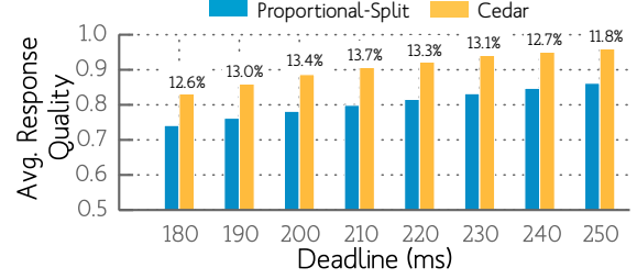
Figure 17: Cedar’s performance with the Gaussian distribution. The percentages on the bars denote the improvement that Cedar provides over Proportional-Split.
