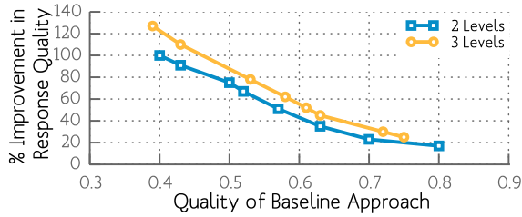
Figure 13: Simulation results showing that Cedar performs even better when the number of levels in the aggregation tree increases. around 55%. Varying the ratio of k_1 over k_2 to over 1 does not change the trend in improvements.
