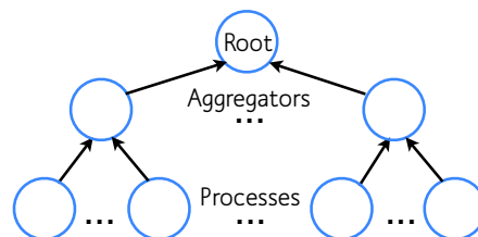
Figure 1: Aggregation Trees. On arrival of a query , computations are spawned across multiple parallel processes whose outputs are combined using aggregators to produce the final response .
