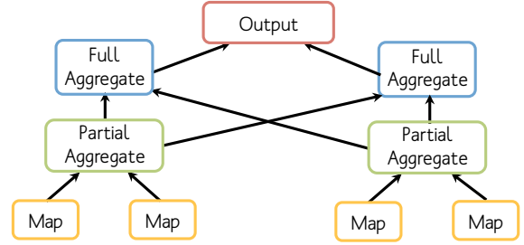
Figure 3: A query to an interactive data analytics system compiled into a DAG of hierarchical parallel processes.
