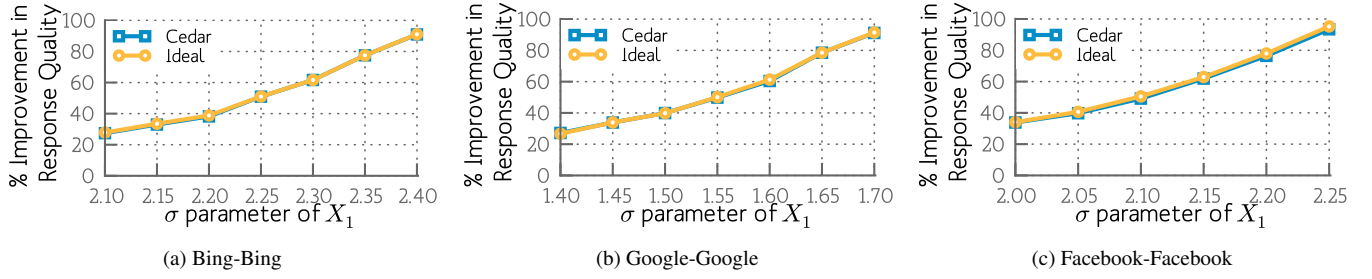
Figure 16: Same Distributions: Percentage Improvement in Response Quality as the \sigma parameter of X_1 is varied. \mu parameter of log-normal distributions X_1 and X_2 and \sigma parameter of X_2 are obtained from (a) Bing, (b) Google, and (c), Facebook distributions.
