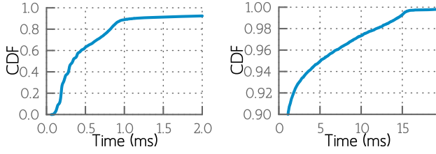
Figure 4: Distribution of RTTs in Bing’s search cluster. The median value is 330\mu s while the 90 th and 99 th percentile values are 1.1ms and 14ms, respectively.
