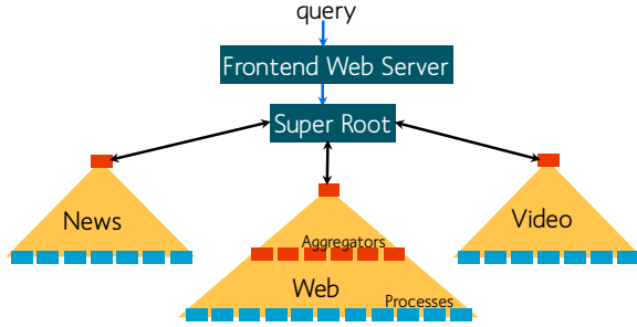
Figure 2: A typical web search computation that aggregates results across many functional silos [13]. The small rectangles at the leaves denote processes of the computation.
