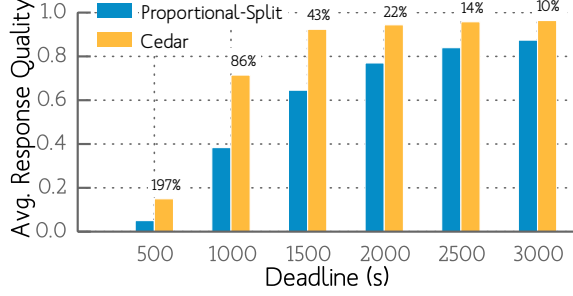
(a) Spark Implementation
