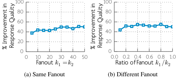
Figure 12: Simulation results showing that Cedar’s gains hold up when the structure of the aggregation tree changes. In (a), we keep the fanout at both the levels. In (b), we choose different fanout for the lower-level while keeping the upper-level fanout at 50. The deadline is set to 1000s.
