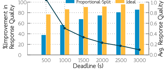
Figure 6: Ideal solution’s improvement in response quality over straw-man solutions for varying deadlines. Distribution X_1 is from the map tasks and X_2 is from the reduce tasks in the Facebook cluster. The fanout is kept constant at 50 (both k_1 and k_2 ) giving a total of 2500 processes.
