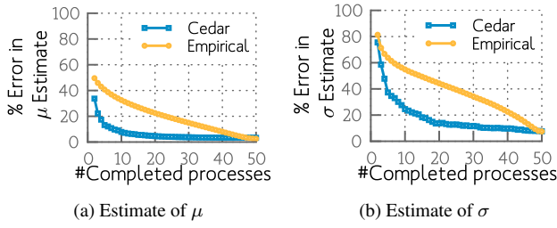
Figure 9: Variation in % error in estimation of the \mu and \sigma parameters of Facebook’s distribution (log-normal with \mu = 2.77 and \sigma = 0.84 ) with the number of responses that have arrived at the aggregator (maximum of 50). The baseline is the empirical estimates for \mu and \sigma from the responses.
