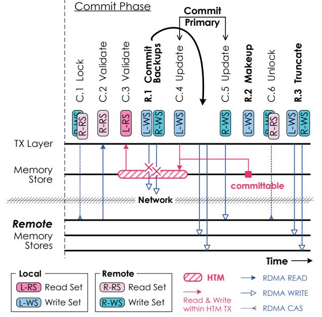
Figure 9. The primary-backup replication in DrTM+R.
