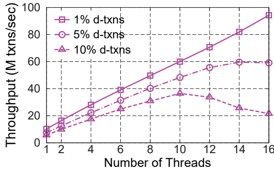
Figure 14. The throughput of standard-mix in SmallBank on DrTM+R with the increase of threads using different probability of cross-machine accesses for SP and AMP .
