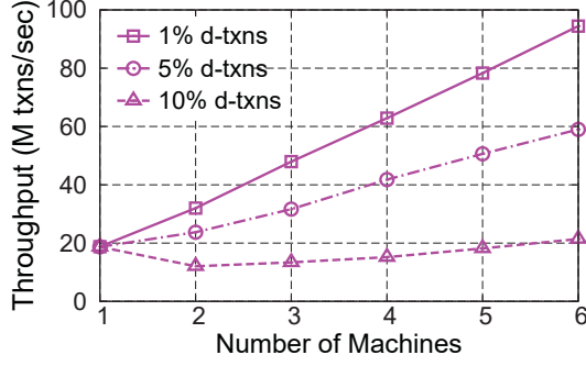
Figure 13. The throughput of standard-mix in SmallBank on DrTM+R with the increase of machines using different probability of cross-machine accesses for SP and AMP .
