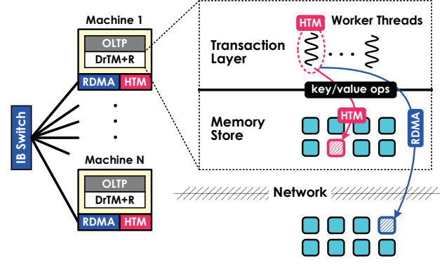
Figure 1. The architecture overview of DrTM+R.
