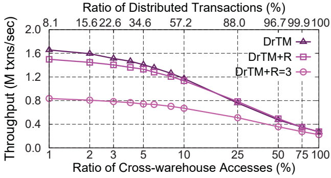
Figure 17. The throughput of new-order transaction in TPC-C with the increase of cross-warehouse accesses while fixing 6 machines and 8 threads each.
