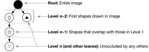
(a) The structure of the compositing-dependence graph for sets of drawing operations.
