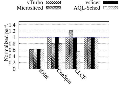
Figure 8. Comparison with other systems: This figure presents the comparison results of our prototype ( AQL_Sched ) with vTurbo, vSlicer, and Microsliced. These results are normalized over the performance obtained with the default Xen scheduler.
