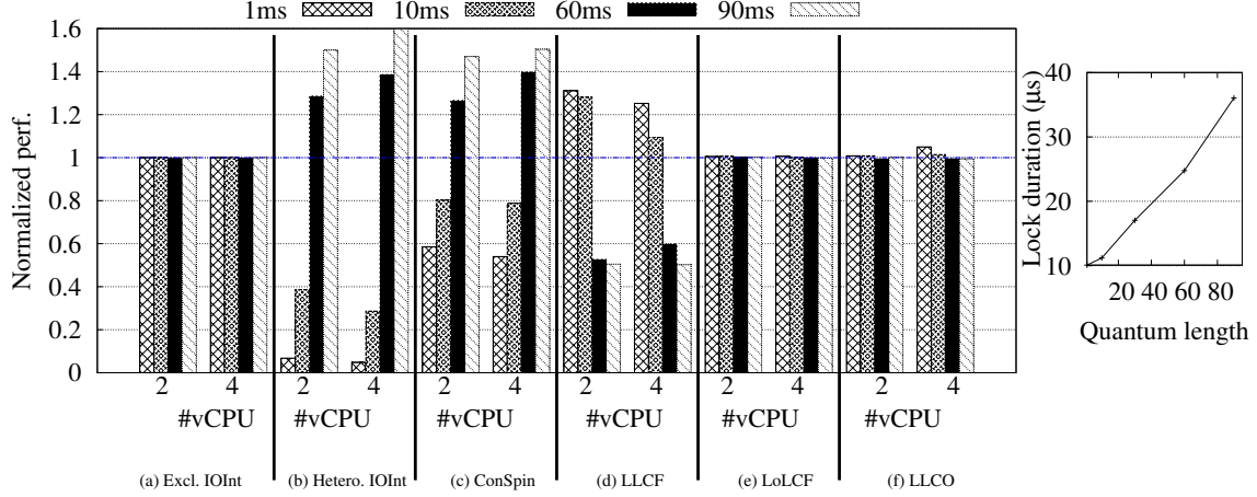
Figure 2. Calibration results: This figure presents the calibration results where values are normalized over the application type performance when it runs with the Xen default quantum length (30ms). The smaller the performance graph bar the better the performance.
