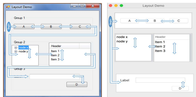
Figure 2. Screen reader navigation models in a typical Windows reader (left), and an OS X reader (right), indicated by arrows. Windows readers, like JAWS, use a “flat” navigation, which cycles through elements in a circularly-linked list. In contrast, VoiceOver on OS X navigates “hierarchically,” effectively traversing a logical tree structure of GUI widgets.
