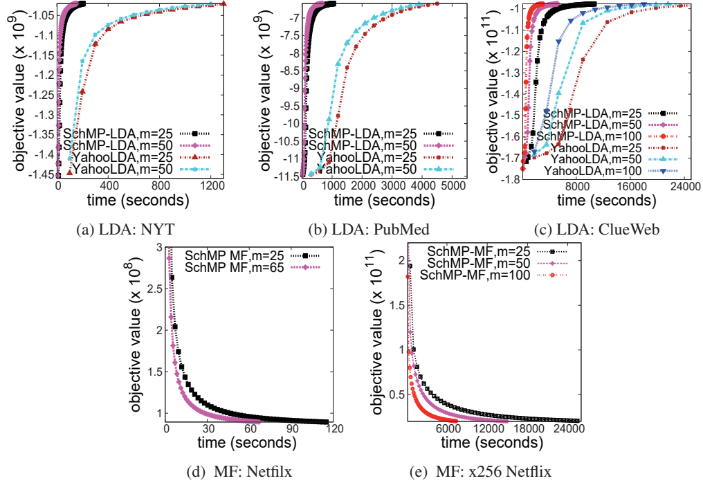
Figure 7: Static SchMP: convergence times. (a-c) SchMP-LDA vs YahooLDA; (d-e) SchMP-MF with varying number of machines m .
