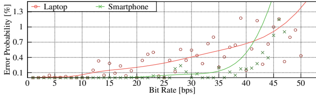
Figure 12. Zoom-in to the low-rate area of Figure 11; showing only the same-core channel.
