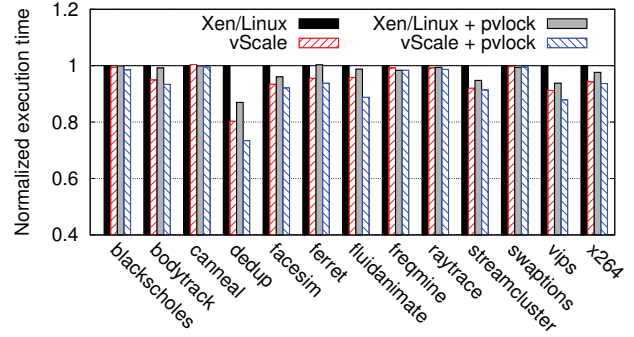
Figure 12: Performance results in PARSEC experiments with an 8-vCPU VM..
