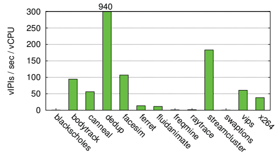
Figure 13: The average IPIs each vCPU received per second in PARSEC experiments, corresponding to Figure 11’s tests.
